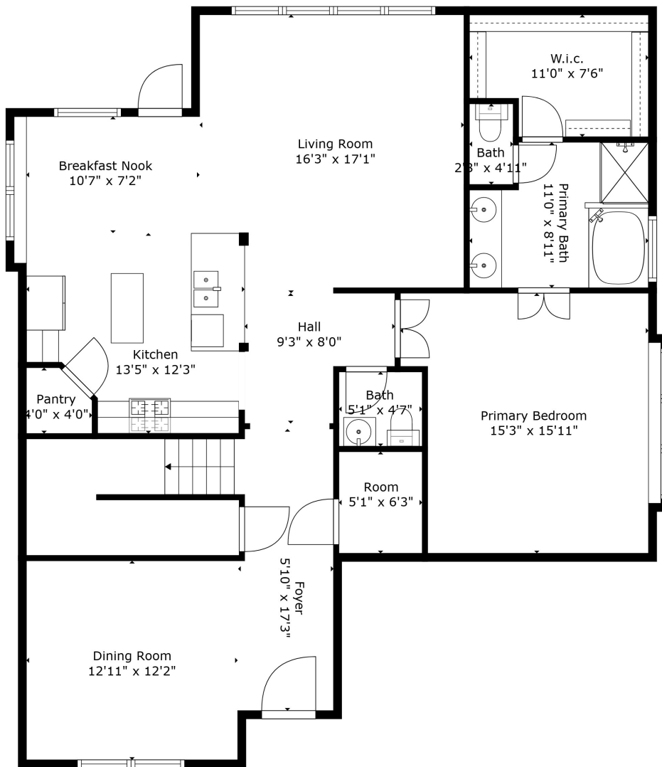
Floor 1
